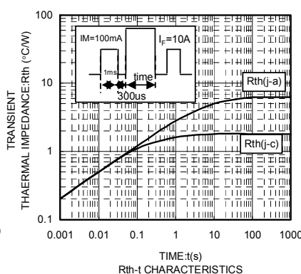
R_{\theta-t} CHARACTERISTICS
